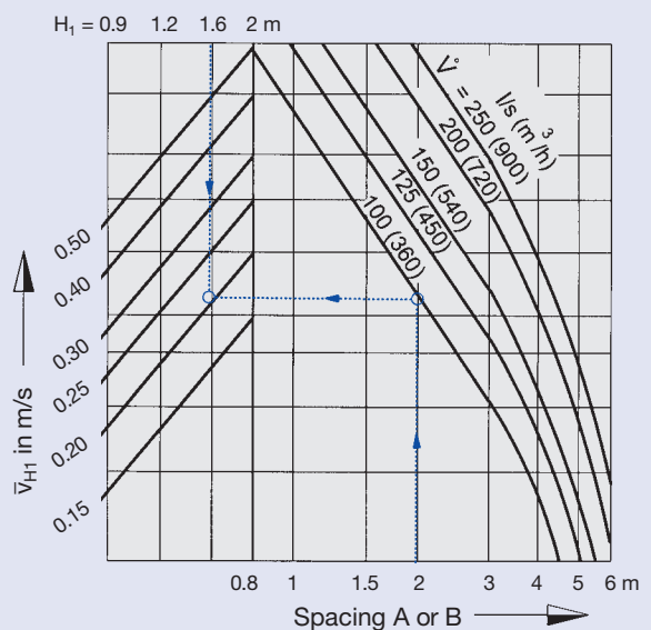
21 Square arrangement of diffusers
