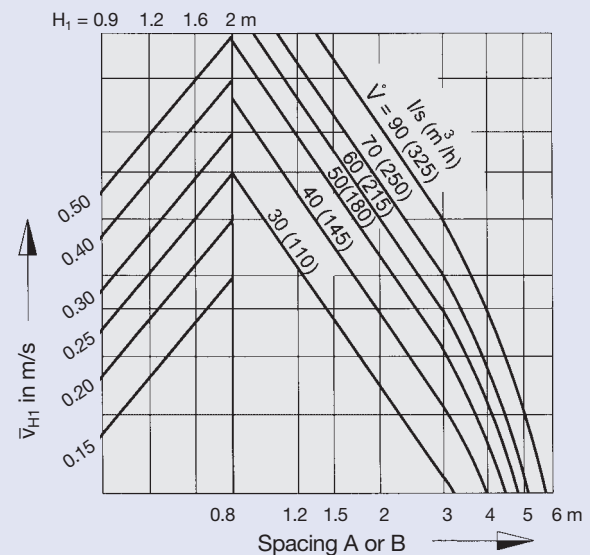
9 Square arrangement of diffusers
