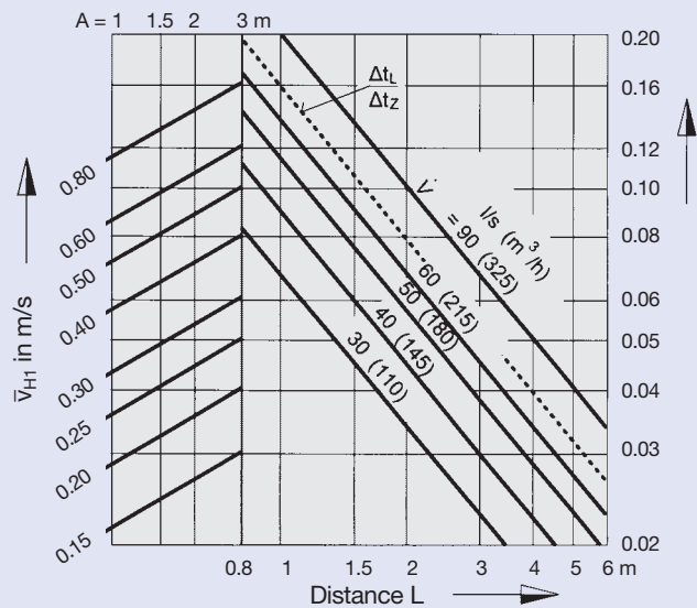
9 Square arrangement of diffusers
