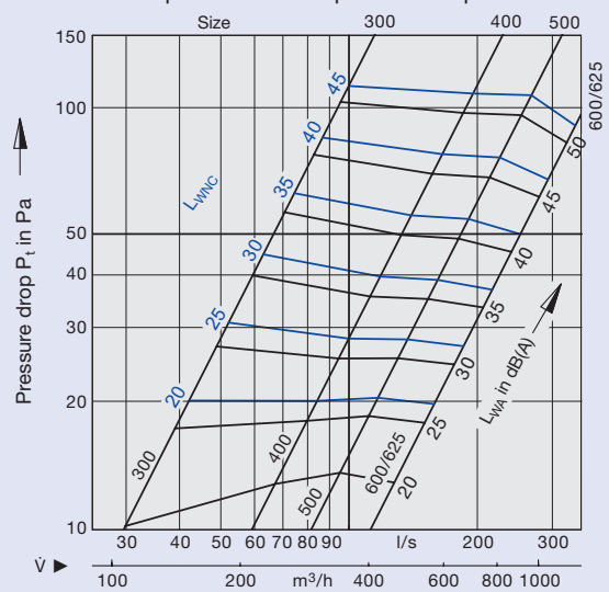
5 TDF-SA-...-H Sound power level and pressure drop
