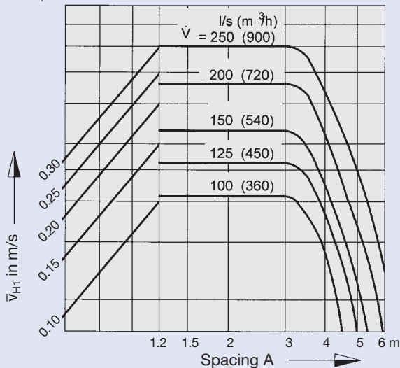
19 Diffuser arrangement: More than one row if B = 3.00 \text{ m} H_1 = 0.9 \text{ 1.2 1.6 2 m}
