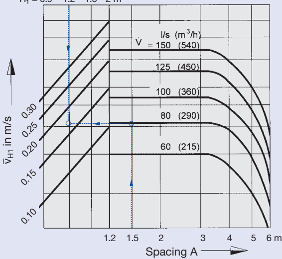
11 Diffuser arrangement: More than one row if B = 3.00 \text{ m} H_1 = 0.9 \ 1.2 \ 1.6 \ 2 \text{ m}
