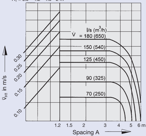
15 Diffuser arrangement: More than one row if B = 3.00 m H_1 = 0.9 \quad 1.2 \quad 1.6 \quad 2 m
