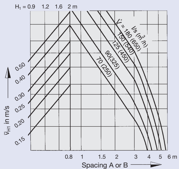
17 Square arrangement of diffusers
