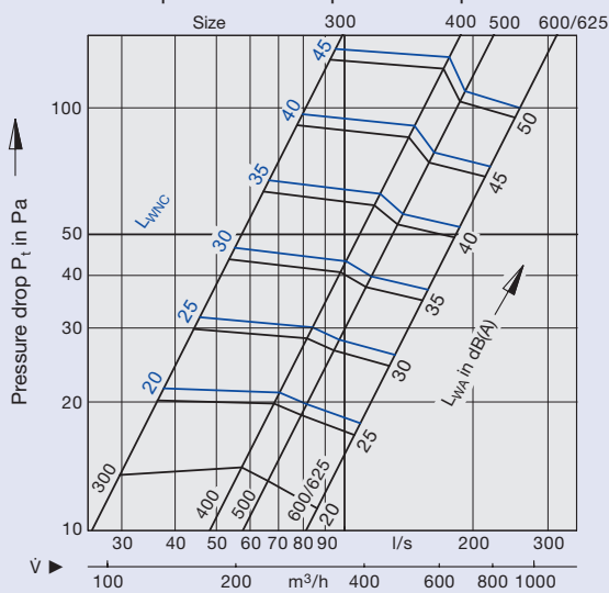
4 TDF-SA-...-V Sound power level and pressure drop
